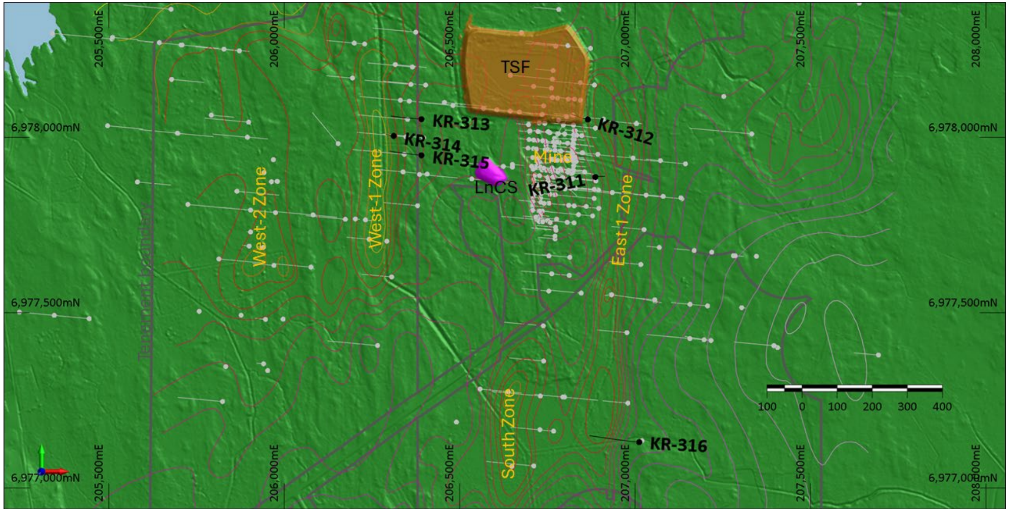
Figure 1: Drill hole location map showing the recently completed holes KR-311 to KR-316. Holes KR-311 and KR-312 targeted near-mine mineralisation, while KR-313, KR-314 and KR-315 tested the mineralised zone west of the mine known as West-1. Hole KR-316 was more exploratory, targeting a gravity and passive seismic anomaly south of the mine. Also shown are the TSF and lanthanide concentrate stockpile locations, gravity contours, previous drilling and the boundaries of European Resources' tenements.
